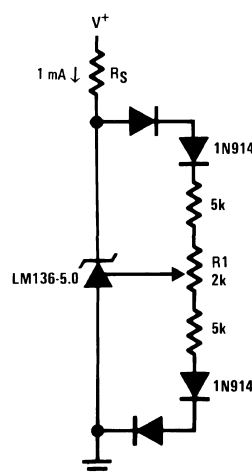
Figure 8. Temperature Coefficient Adjustment (Trim Range = \pm 0.5\text{V} Typical)
