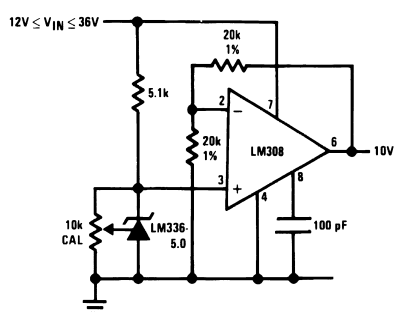
Figure 16. 10V Buffered Reference
