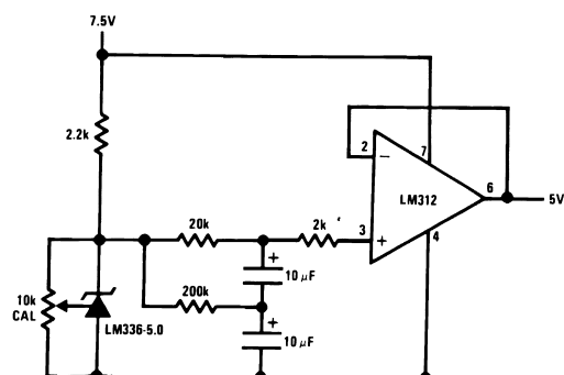
Figure 17. Low Noise Buffered Reference
