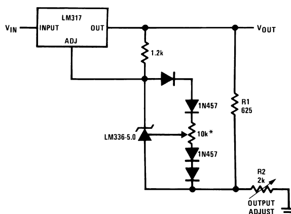
Figure 9. Precision Power Regulator with Low Temperature Coefficient
