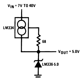
Figure 18. Wide Input Range Reference
