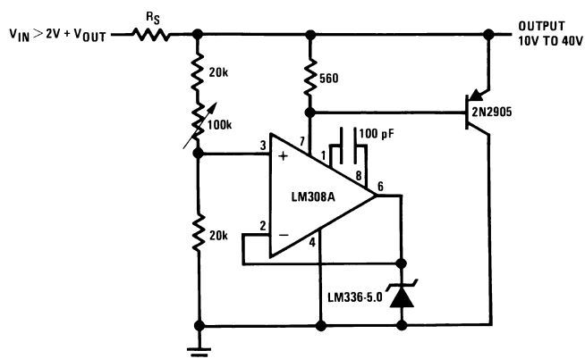
Figure 11. Adjustable Shunt Regulator
