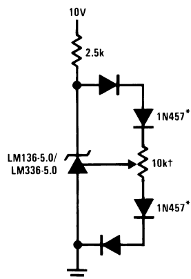
Figure 4. 5.0V Reference
