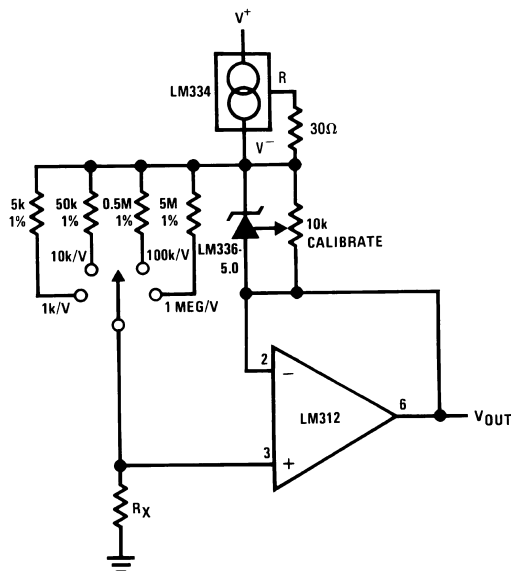
Figure 12. Linear Ohmmeter
