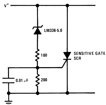
Figure 10. 5V Crowbar
