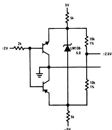
Figure 14. Bipolar Output Reference
