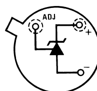
Figure 2. TO-46 Metal Can Package (Bottom View)
