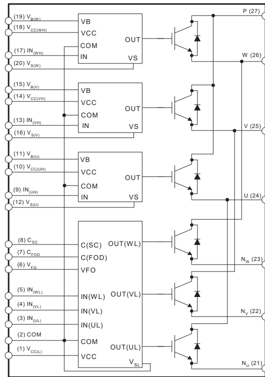
Figure 3. Internal Block Diagram
