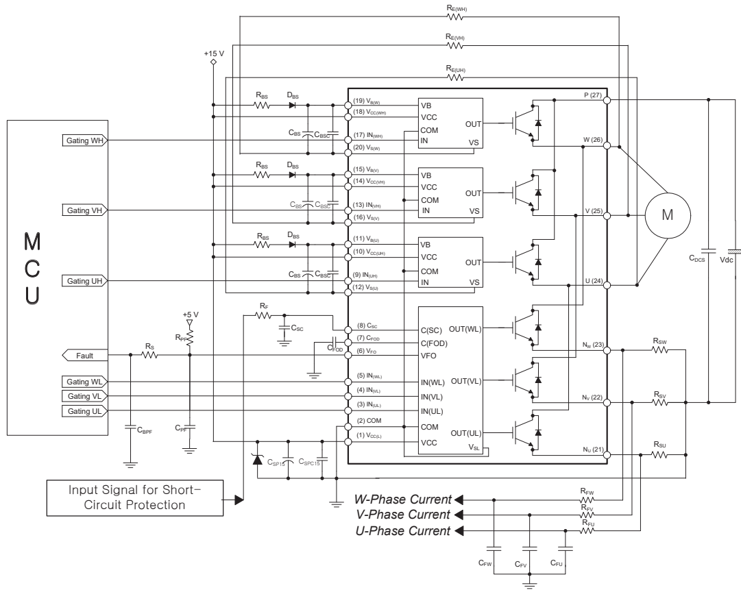
Figure 11. Typical Application Circuit
