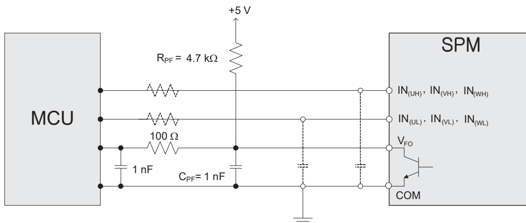
Figure 9. Recommended MCU I/O Interface Circuit
