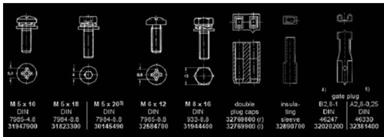
Fig.6-2 Mounting screws for SEMIPACK Modules
