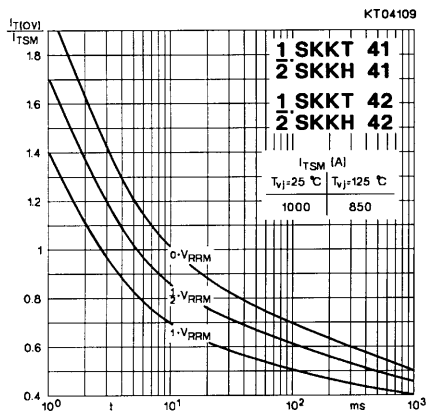
Fig. 9 Surge overcurrent current vs. time
