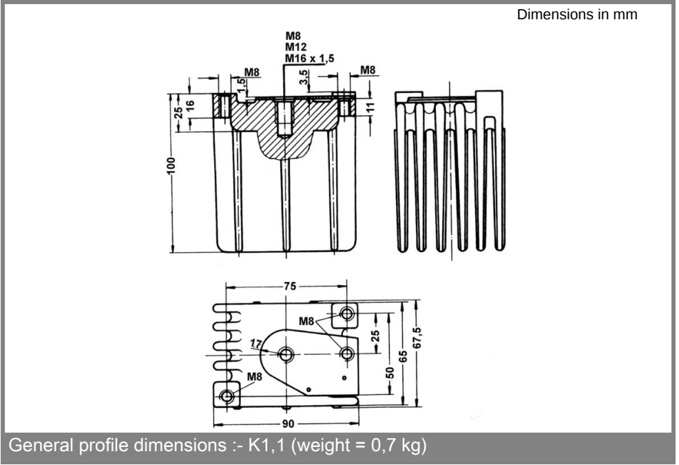
Heatsink
