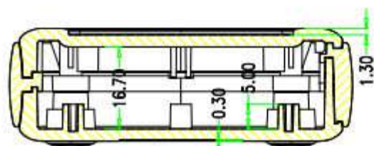
SEC B-B
